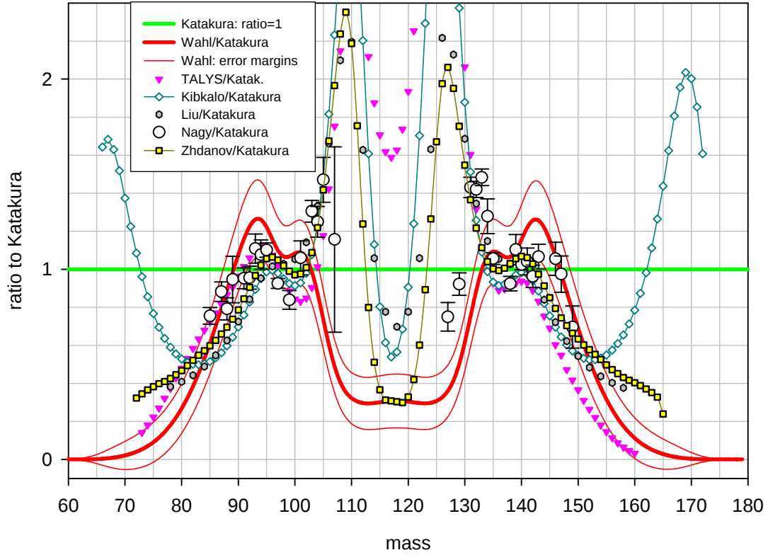
Benchmark A: ^{238}\text{U} at 5.5 MeV, post neutron emission yield ratios to Katakura's systematics lower graph: partial plot (very high and low values omitted)
